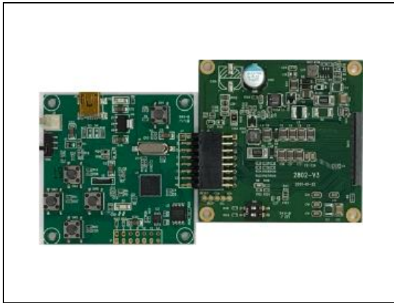
MCU board and display adapter
